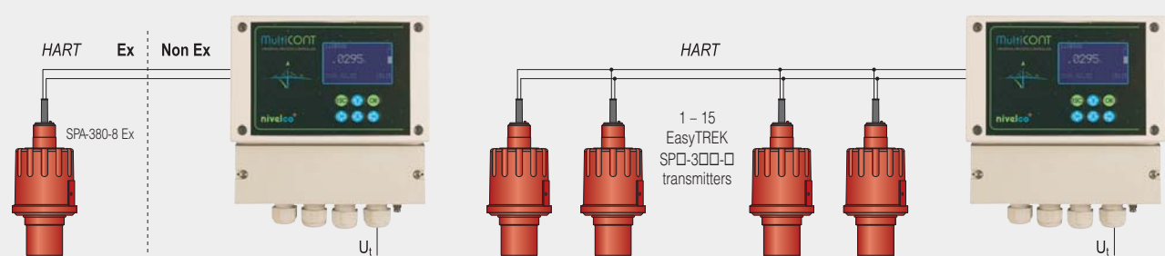
Multicont powering an EasyTREK in a hazardous area
